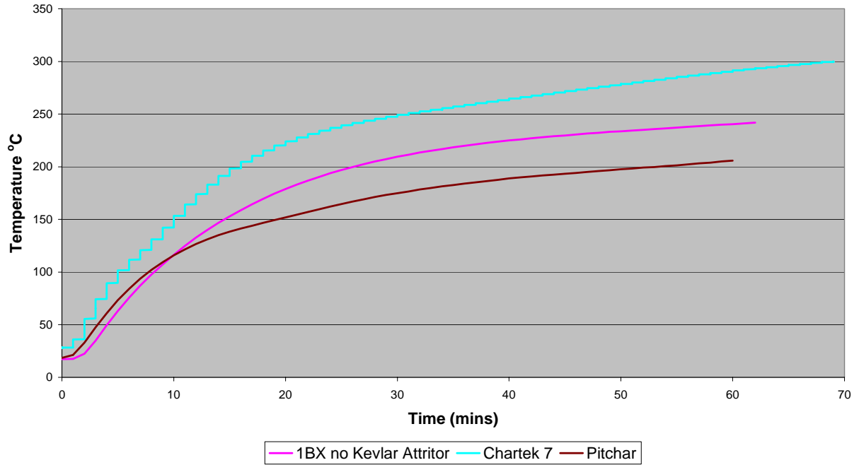
Jetfire test of current products against PD70
