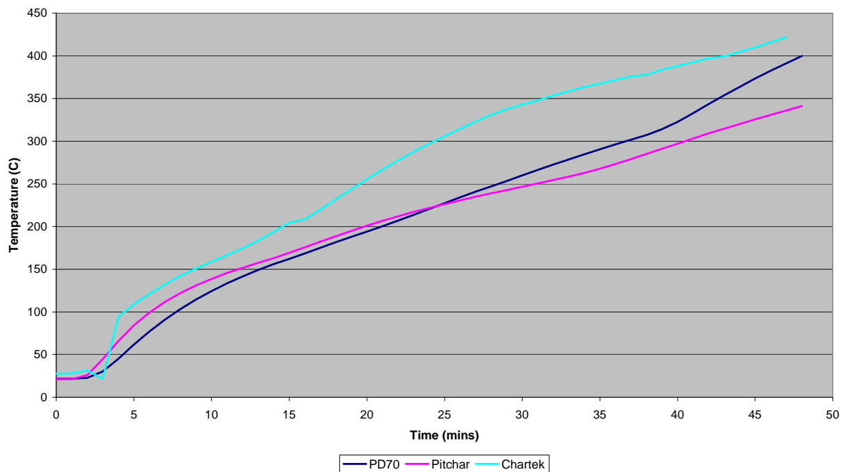
Engulfment test of offshore competitive products
