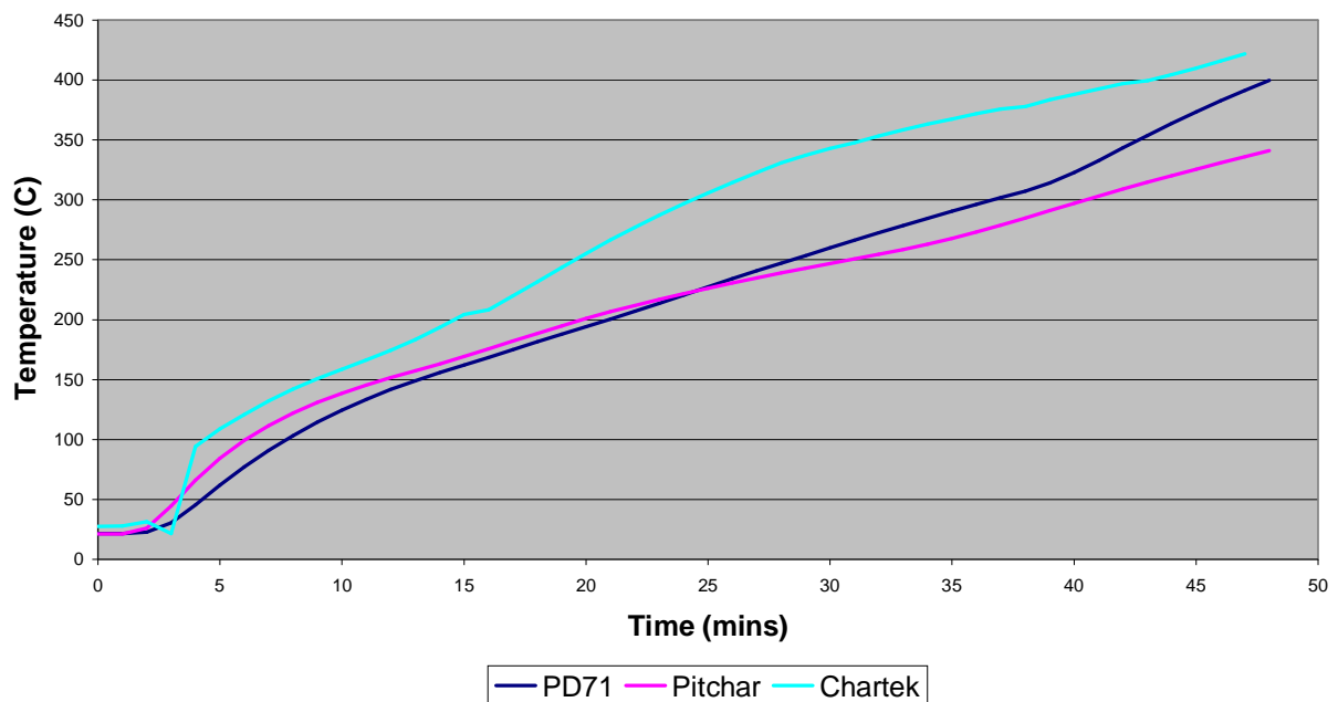
Engulfment test of offshore competitive products
